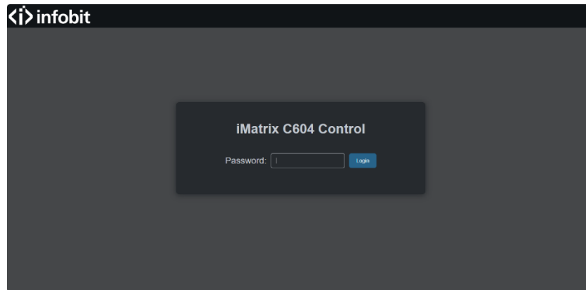
Figure 7: Login Window
