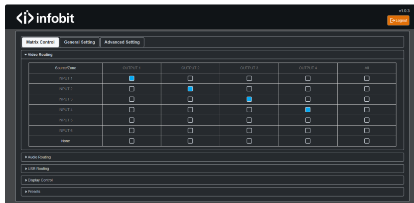
Figure 9: Main Page
