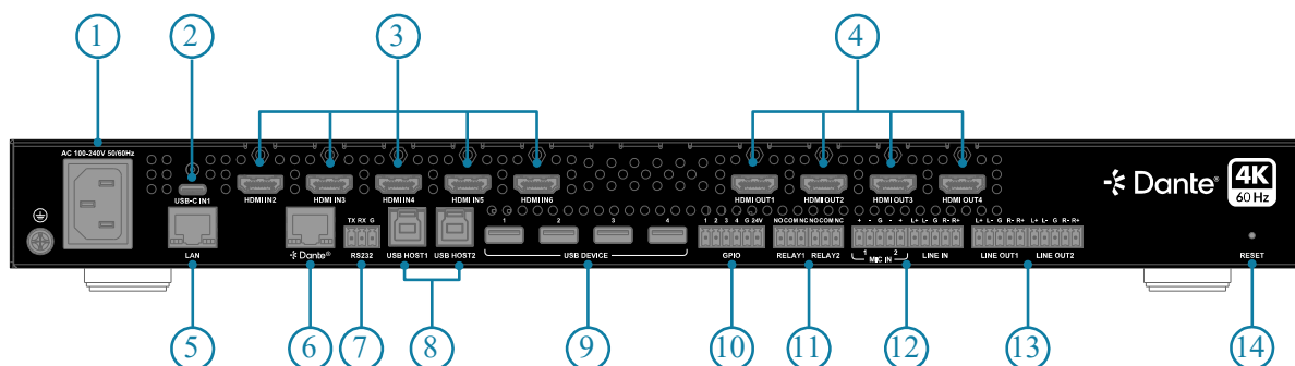
Figure 2: Rear Panel
