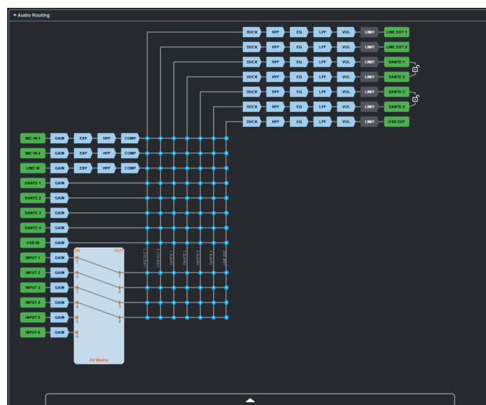
Figure 11: Audio Routing
