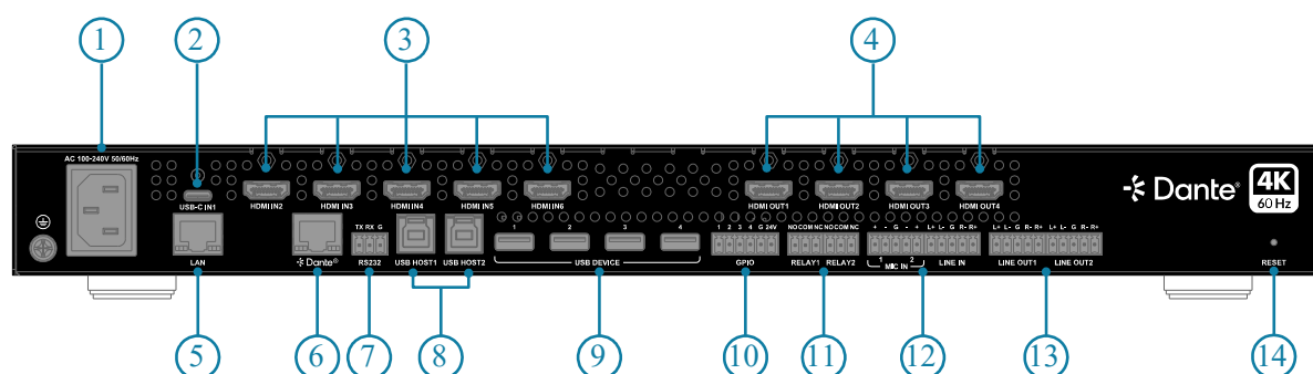
Figure 2: Rear Panel
